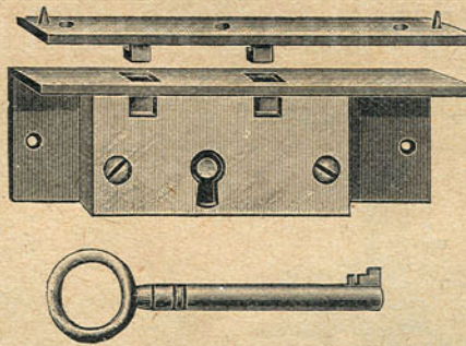
No. 2. BOX LOCK. BEST LEVER. Size 2 in. Price 1/6 Post free 1/7
